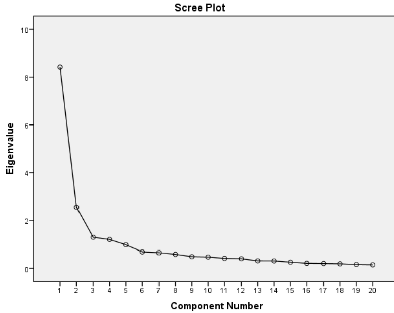
Graph 1: Scree Plot
